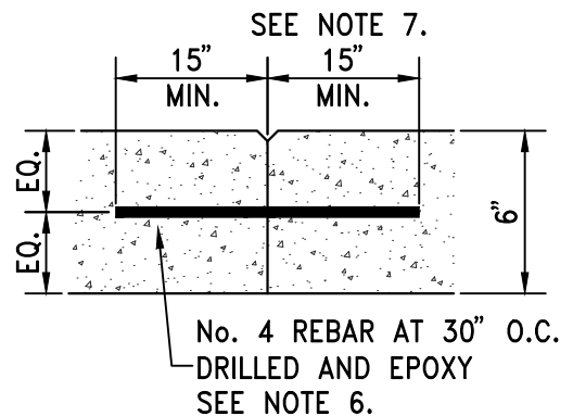
DETAIL B (CONSTRUCTION JOINT)
